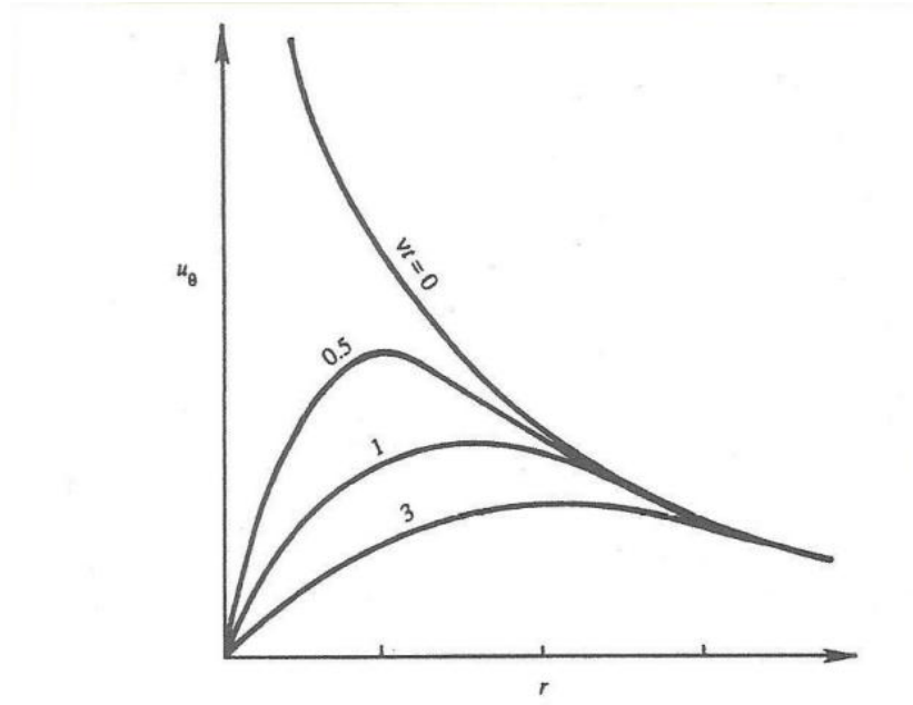
Figure 9.12 Viscous decay of a line vortex showing the tangential velocity at different times.
