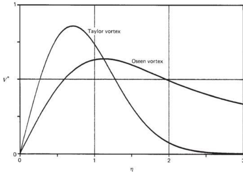
Figure 11.8 Profiles for Oseen and Taylor vortices in similarity variables. For the Oseen vortex, V^* \propto v_{\theta}/t^{-1/2} , while for the Taylor vortex, V^* \propto v_{\theta}/t^{-3/2} . In each case \eta = r/\sqrt{\nu t} .
