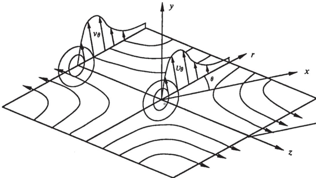
Figure 11.11 Burgers vortex.
