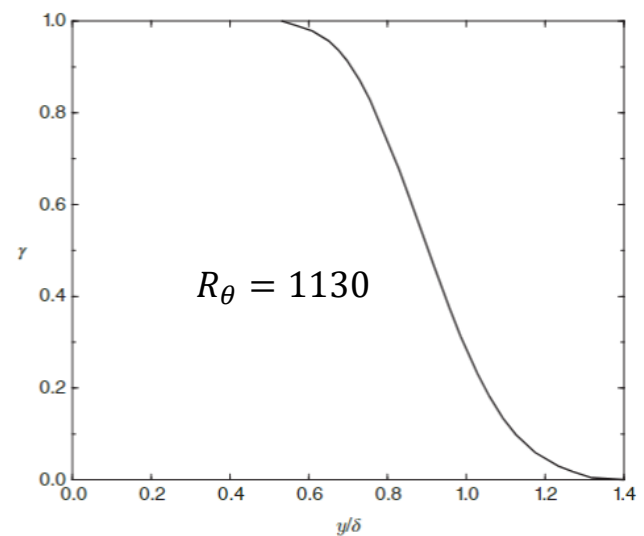
Figure 8.4 Intermittency factor in a turbulent boundary layer [5].
