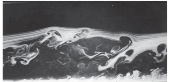
Figure 8.2 Smoke visualization of a turbulent boundary layer at Re_\theta = 3000 [1].
