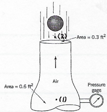
FIGURE P9.78
